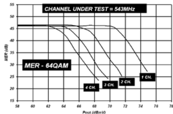
Figure 24b: ACA1206 MER – 64 QAM @ 543 MHz ( I DD = 325 mA)
