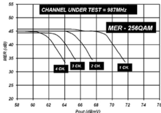
Figure 24f: ACA1206 MER – 256 QAM @ 987 MHz ( I DD = 325 mA)
