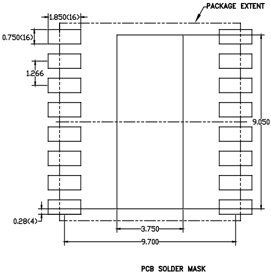
Figure 33: PCB Pad Layout and Solder Mask Detail
