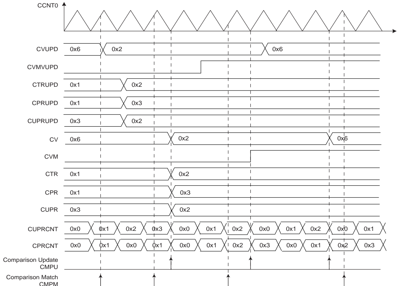
Figure 38-14. Comparison Waveform
