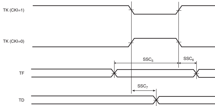
Figure 43-19. SSC Transmitter, TK and TF as input
