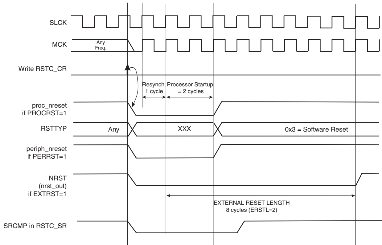
Figure 16-5. Software Reset
