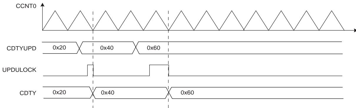
Figure 38-9. Method 1 (UPDM = 0)
