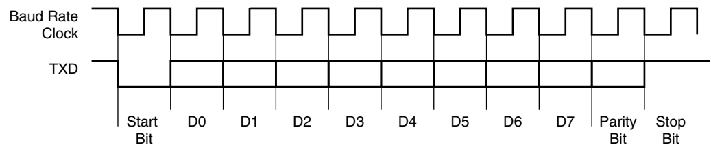
Figure 35-6. Character Transmit
