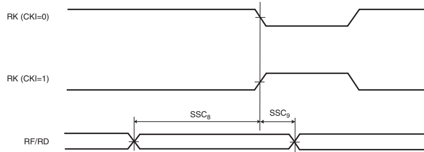
Figure 43-20. SSC Receiver RK and RF as input
