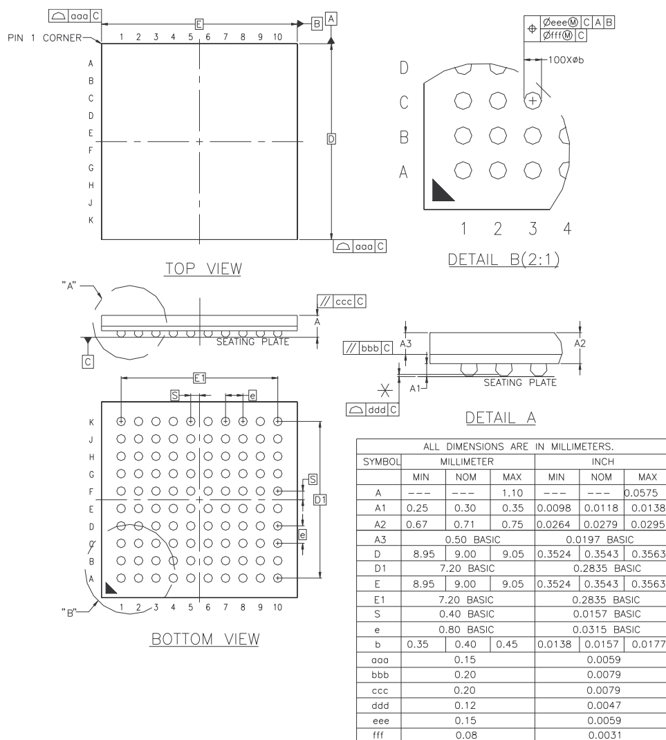
Figure 44-2. 100-ball TFBGA Package Drawing
