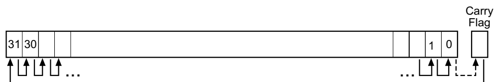
Figure 13-8. RRX
