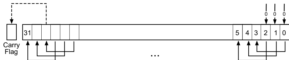
Figure 13-6. LSL #3
