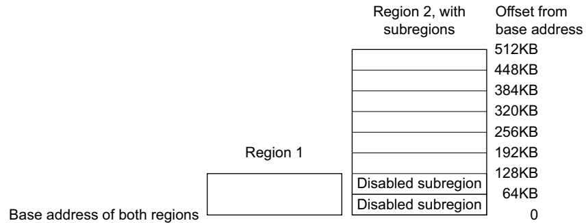
Figure 13-9. SRD use
