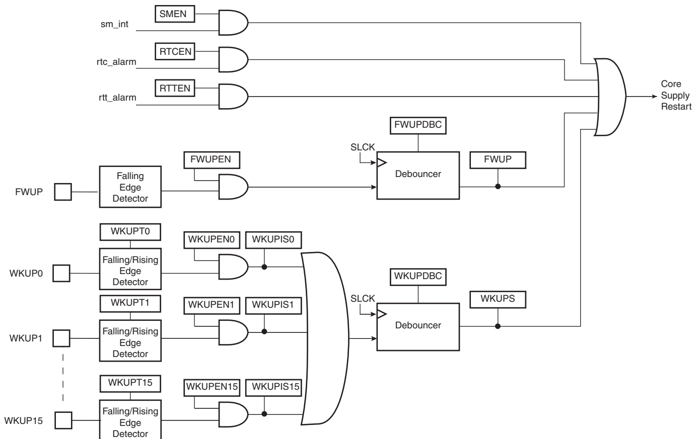
Figure 19-7. Wake Up Sources
