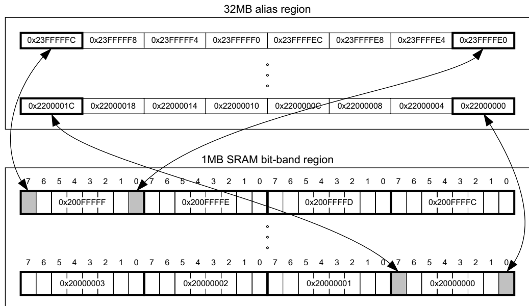
Figure 13-2. Bit-band mapping
