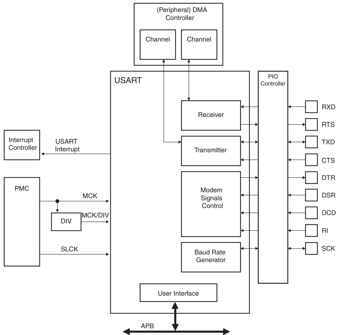
Figure 35-1. USART Block Diagram
