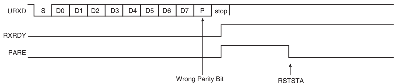
Figure 34-7. Parity Error
