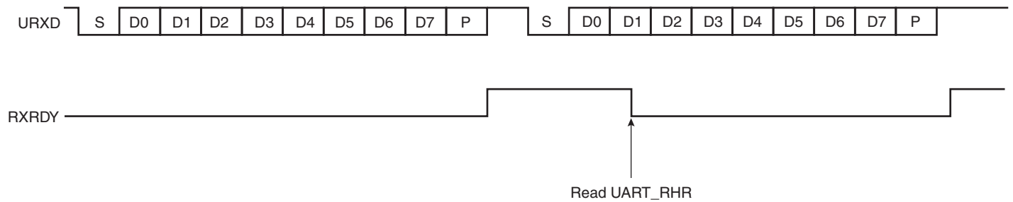
Figure 34-5. Receiver Ready
