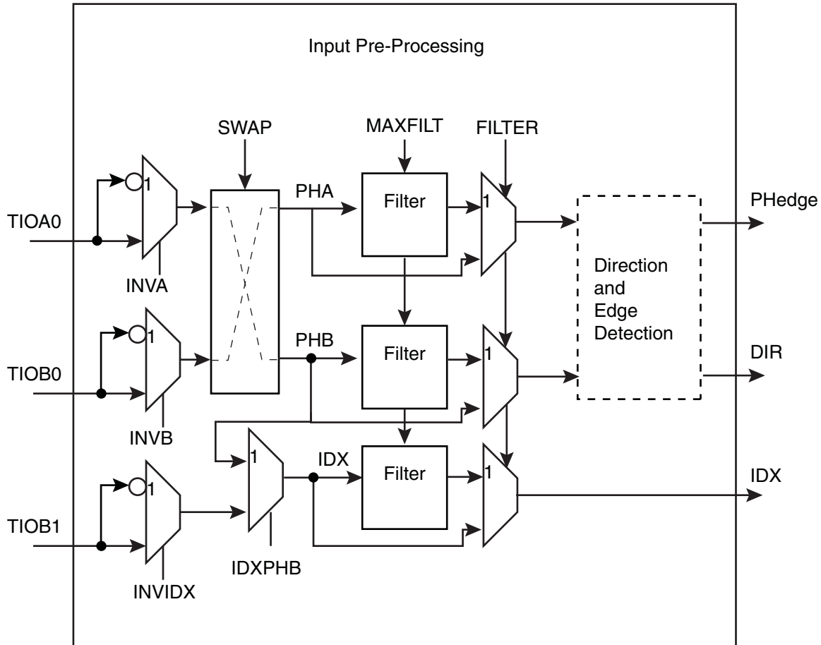
Figure 36-16. Input Stage
