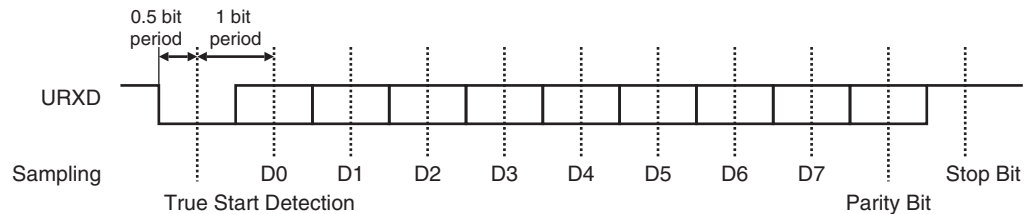
Figure 34-4. Character Reception
