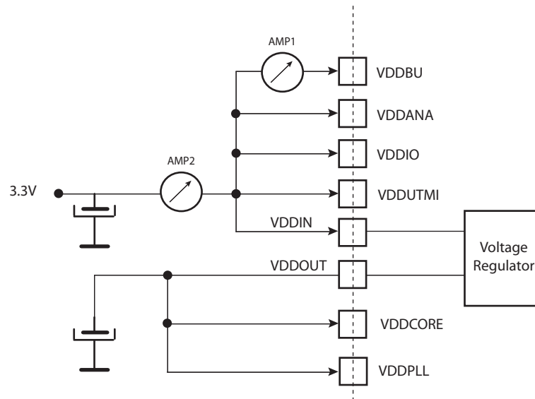
Figure 43-5. Measurement Setup
