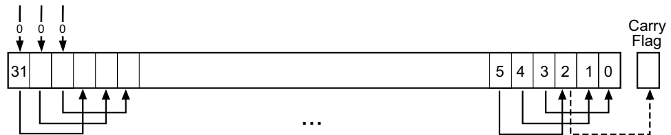
Figure 13-5. LSR #3
