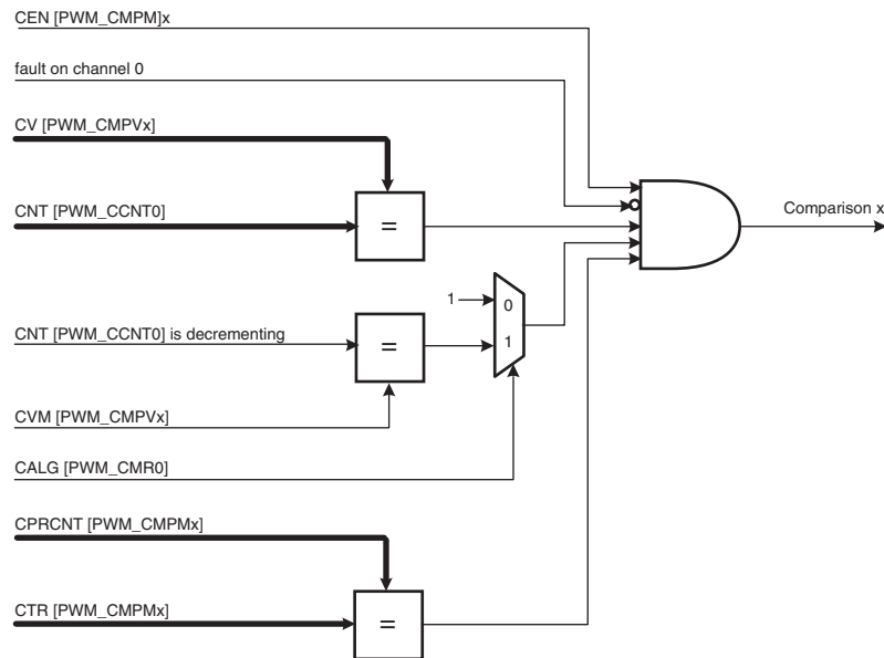
Figure 38-13. Comparison Unit Block Diagram
