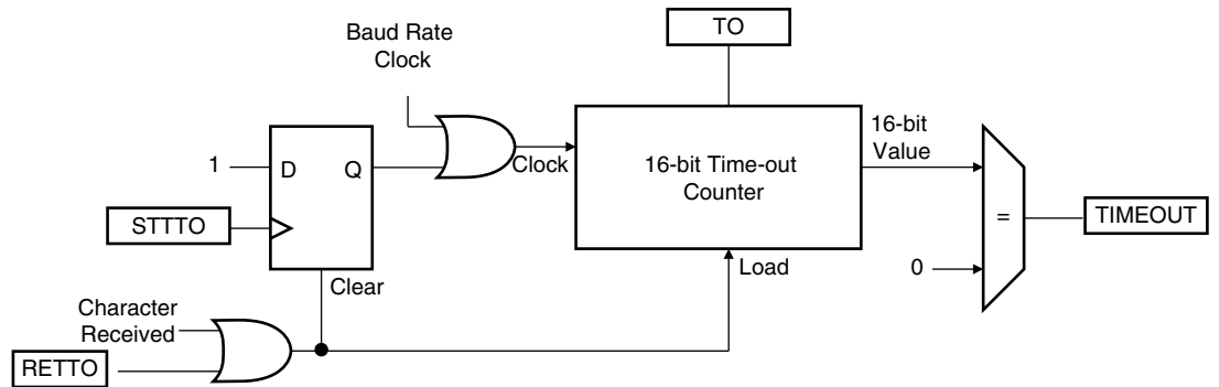
Figure 35-24. Receiver Time-out Block Diagram
