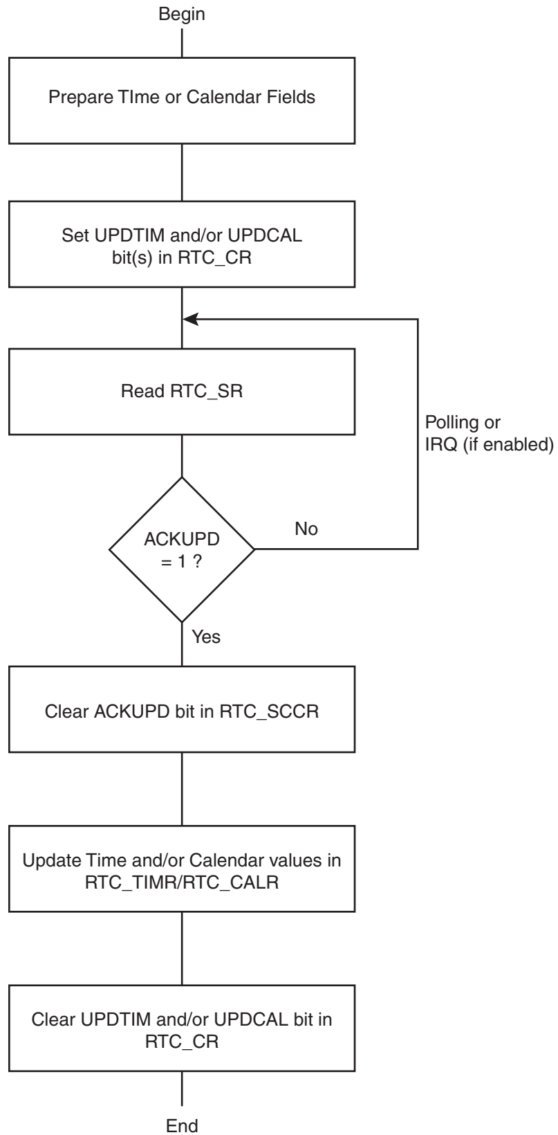
Figure 18-2. Update Sequence
