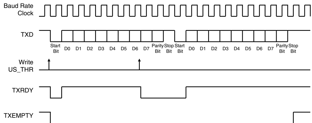
Figure 35-7. Transmitter Status
