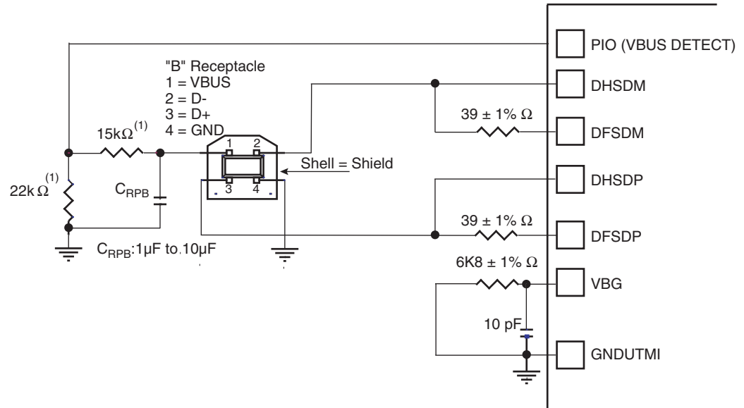
Figure 39-2. Board Schematic
