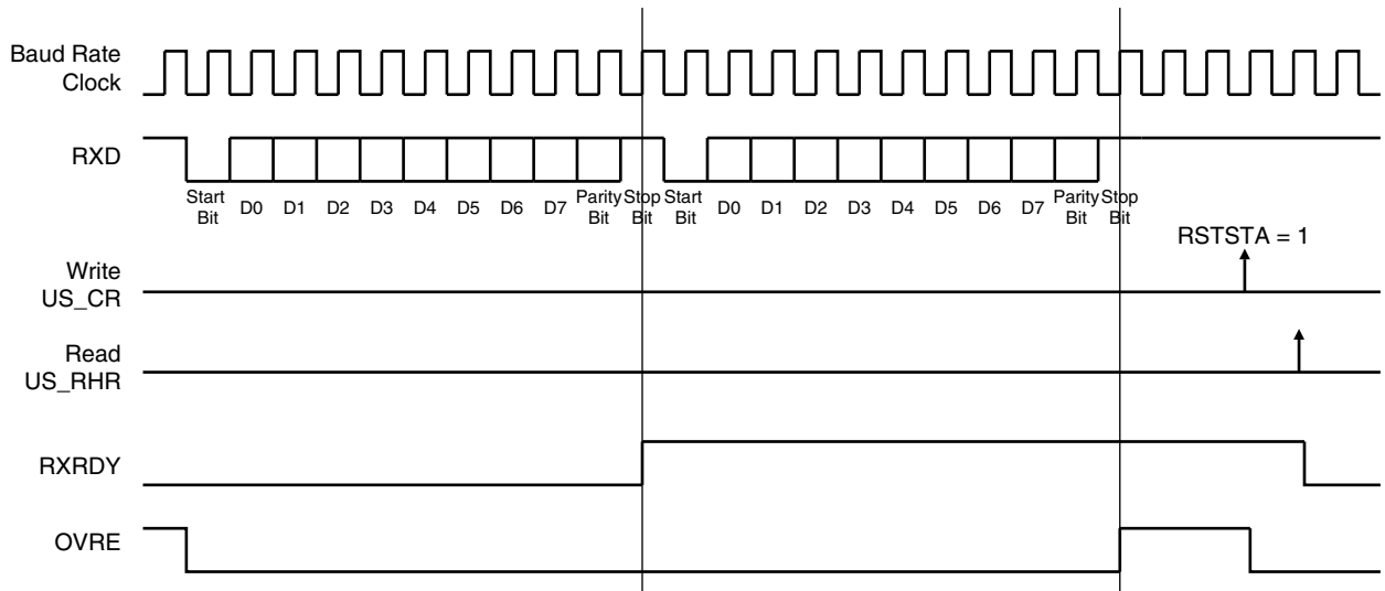
Figure 35-21. Receiver Status
