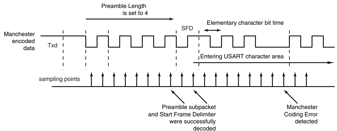
Figure 35-16. Manchester Error Flag
