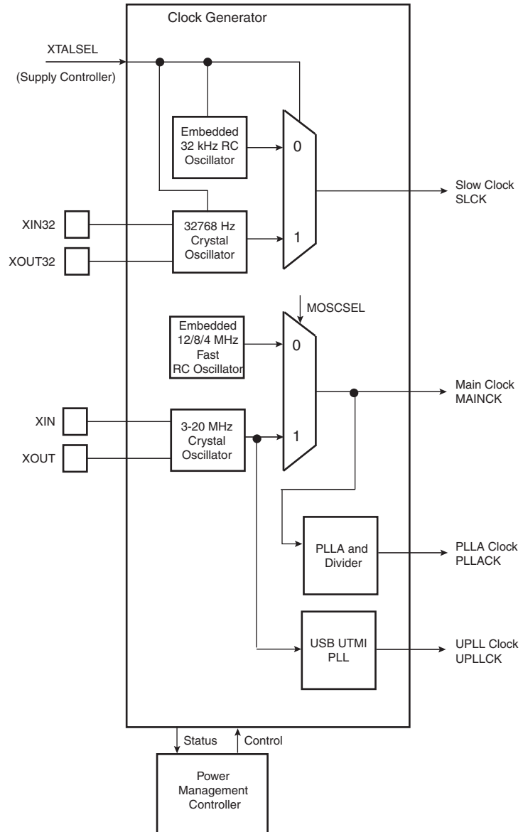
Figure 27-1. Clock Generator Block Diagram
