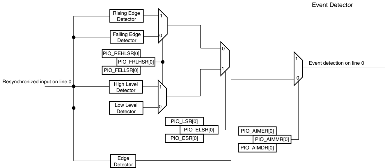
Figure 30-7. Event Detector on Input Lines (Figure represents line 0)
