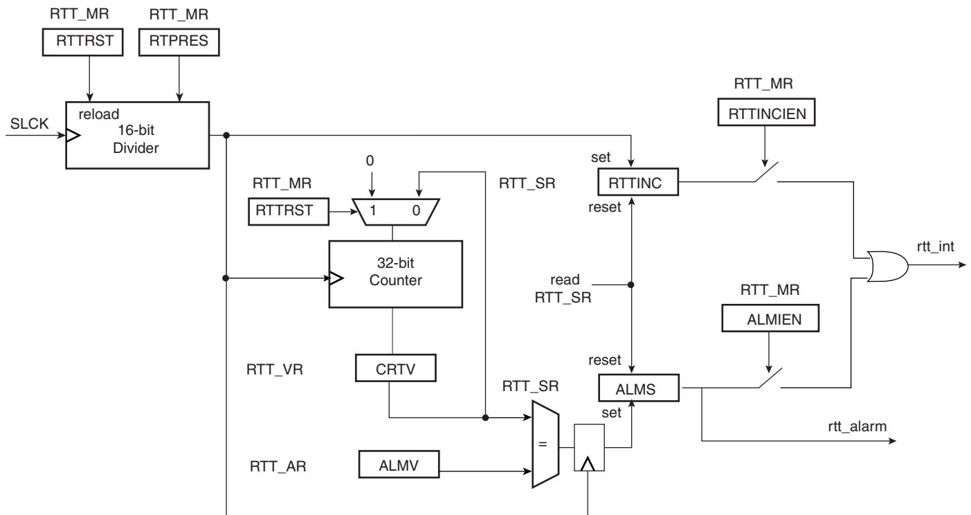
Figure 17-1. Real-time Timer
