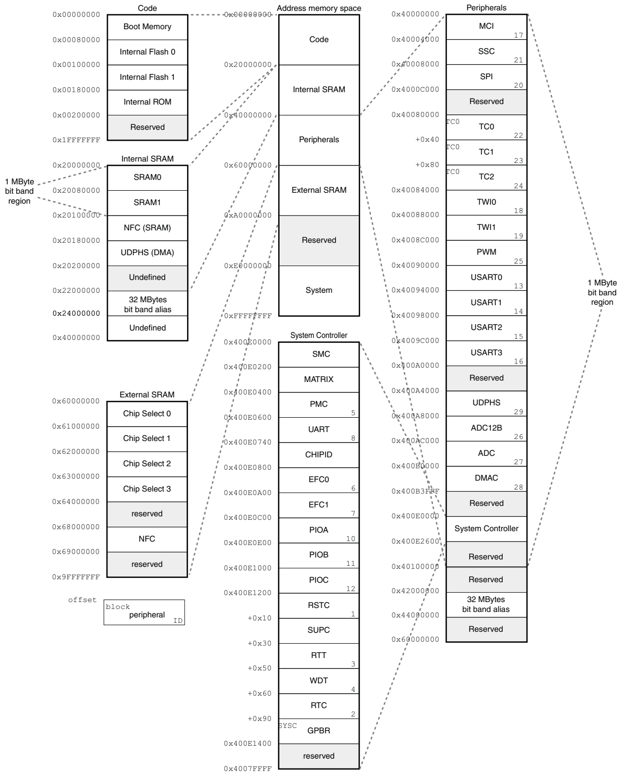
Figure 8-1. ATSAM3U4/2/1 Memory Mapping
