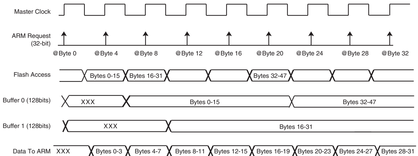
Figure 21-2. Code Read Optimization for FWS = 0
