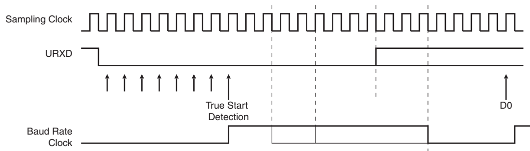
Figure 34-4. Character Reception
