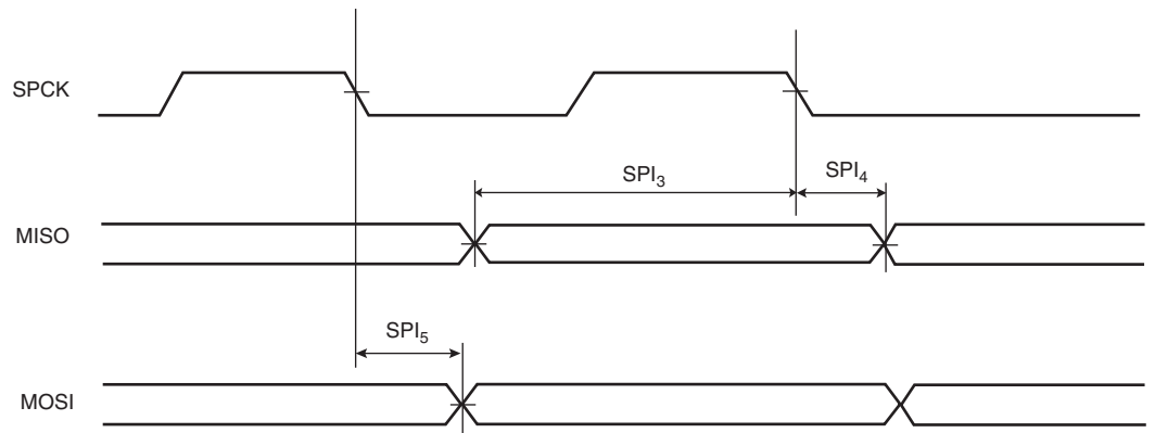
Figure 43-13. SPI Master Mode with (CPOL = 0 and NCPHA=1) or (CPOL=1 and NCPHA= 0)
