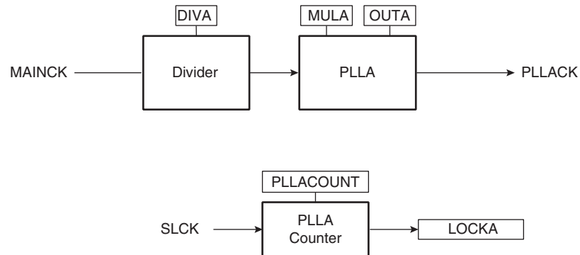
Figure 27-4. Divider and PLLA Block Diagram
