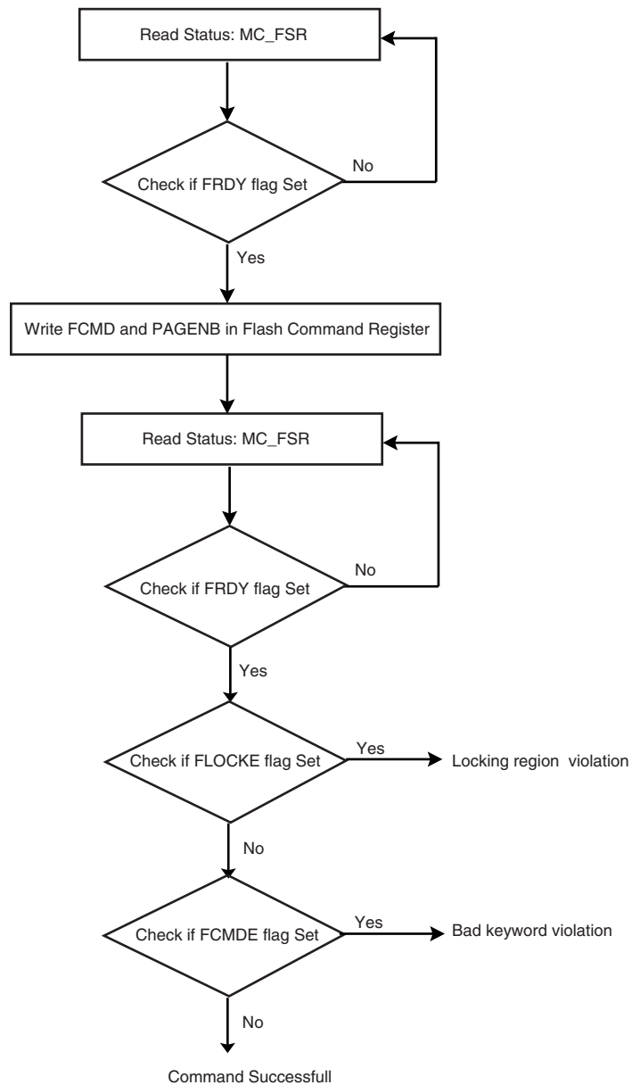
Figure 21-5. Command State Chart
