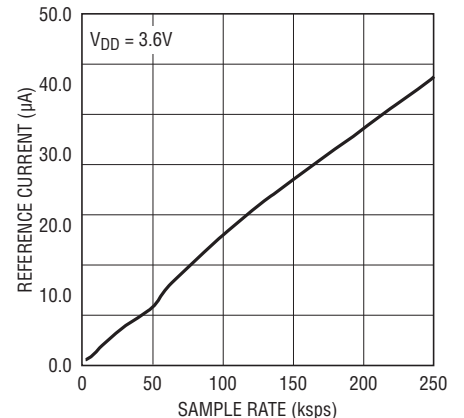
Reference Current vs Sample Rate (TS8 Package)
