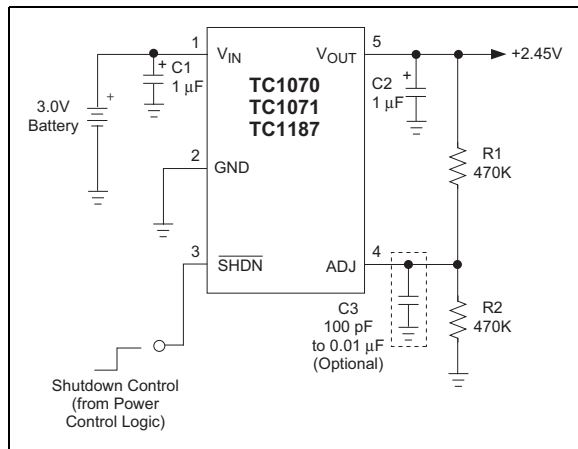
FIGURE 4-1: Battery-Operated Supply
