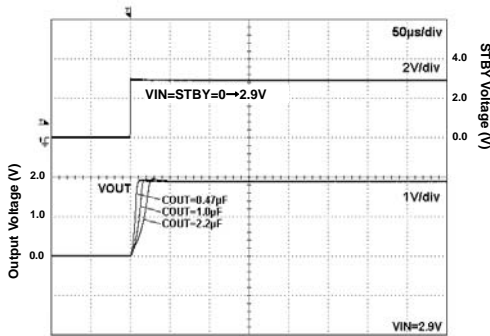
Fig 99. Start Up Time (VIN=STBY) Iout=0mA
