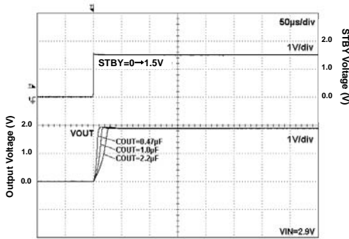
Fig 97. Start Up Time Iout=0mA
