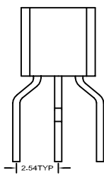
SOT54 LEAD BEND L01 Bulk Pack - 412
