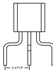
SOT54 LEAD BEND L02 Bulk Pack - 412
