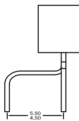
SOT54 LEAD BEND L01 Bulk Pack - 412
