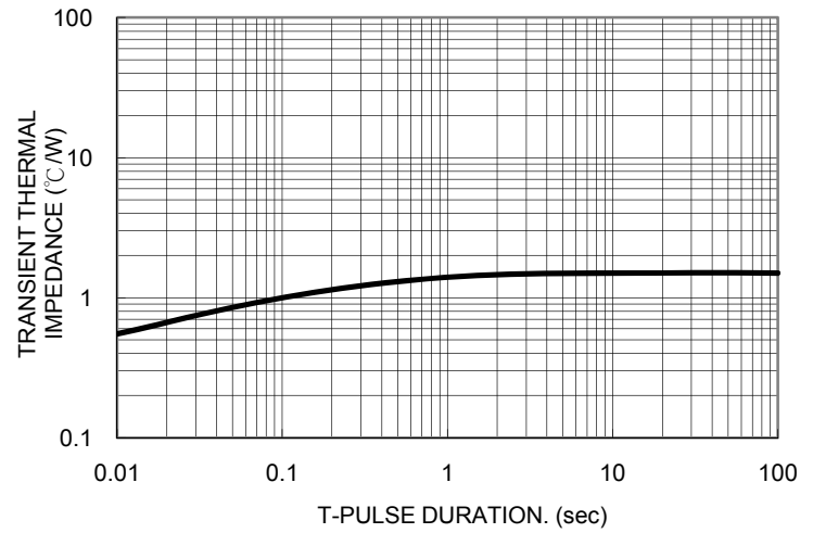
FIG. 6- TYPICAL TRANSIENT THERMAL CHARACTERISTICS PER LEG
