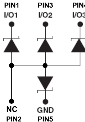
Figure1: UESD6V8L4B use as three bidirectional lines protector
