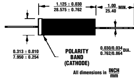
FIGURE 1 DESIGN DATA
