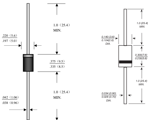
DO-201AE
