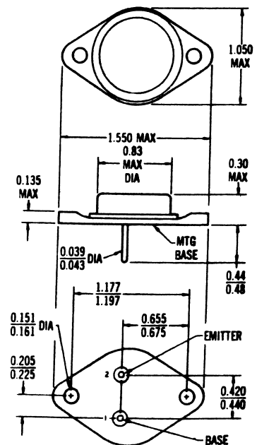
TO-3 Package
