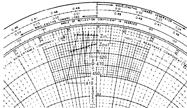
INPUT/OUTPUT IMPEDANCE
