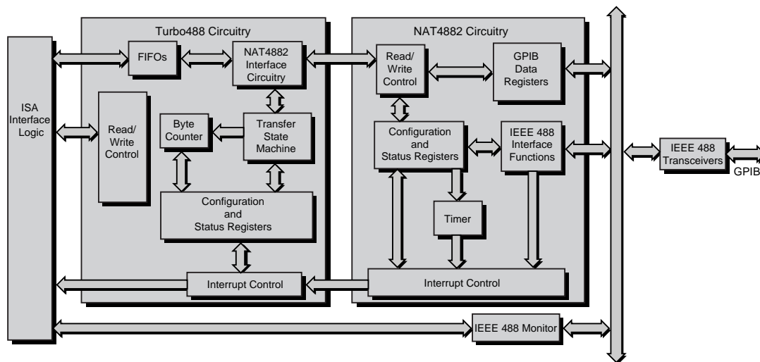
Figure 2. TNT4882 Two-Chip Mode
