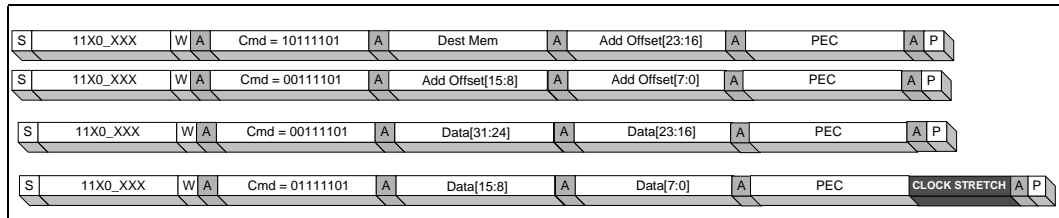
Figure 2-9. Word Configuration Write Protocol (SMBus Byte Write, PEC Enabled)
