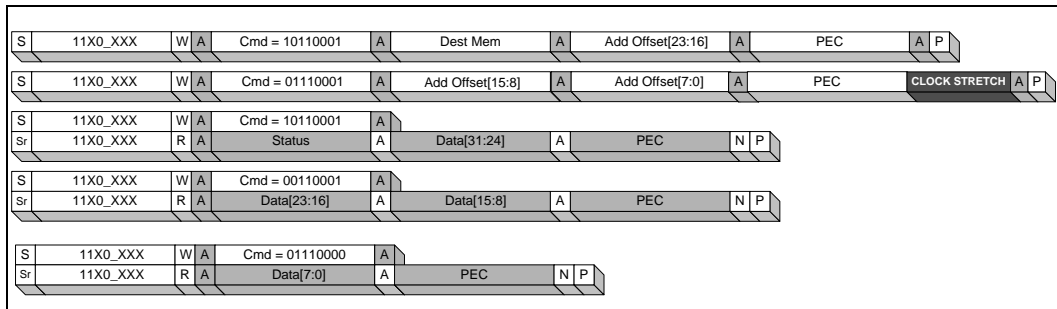
Figure 2-11. DWord Memory Read Protocol (SMBus Word Write/Byte Read, PEC Enabled)
