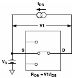
Test Circuit 1. On Resistance Figure 2. Test Circuit 1. On Resistance
