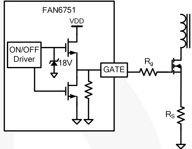
Figure 21. Gate Driver
