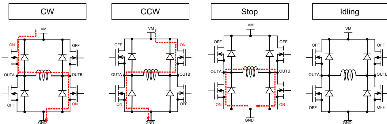
Figure 4. H-Bridge Driver Operation Status
