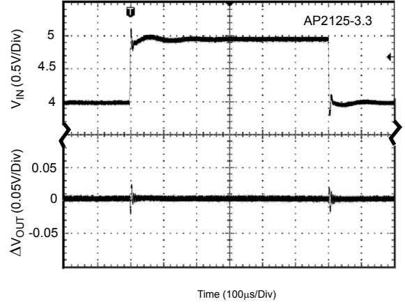
Figure 29. Line Transient (Conditions: I_{OUT}=30mA , C_{OUT}=1\mu F , V_{IN}=4 to 5V )
