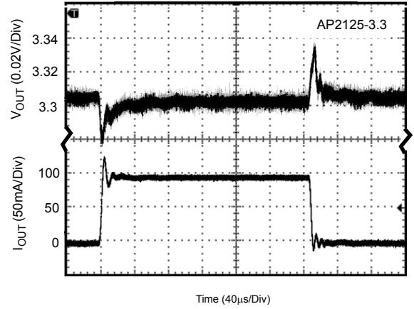
Figure 31. Load Transient (Conditions: I_{OUT}=10 to 100mA , C_{IN}=1\mu F , C_{OUT}=1\mu F , V_{IN}=4.3V )
