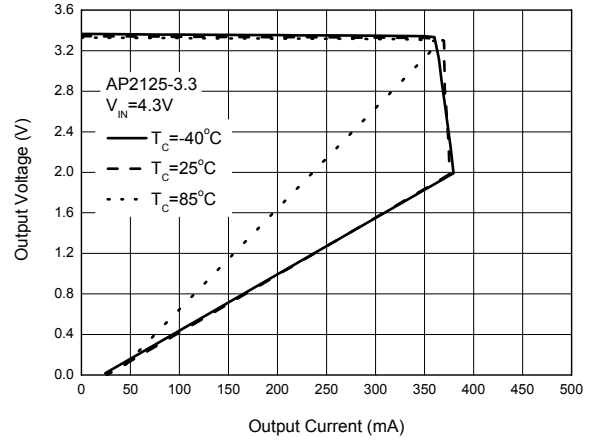
Figure 13. Current Limit
