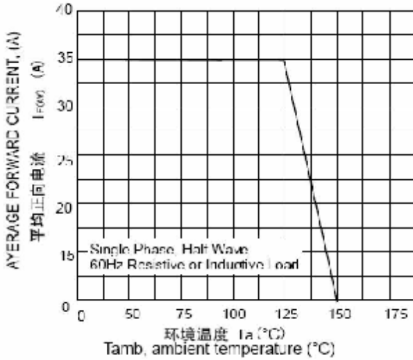
FIG. 1 – DERATING CURVE FOR OUTPUT RECTIFIER CURRENT
