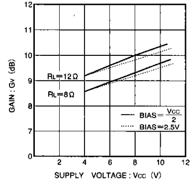
Fig. 10 Driver supply voltage vs. voltage gain
