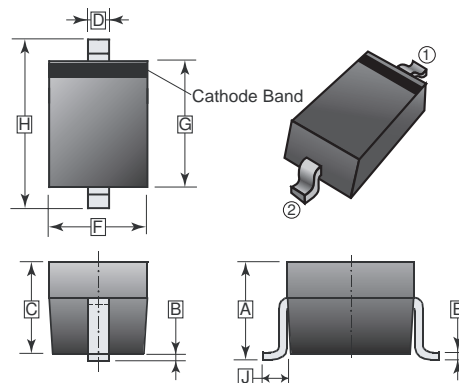
SOD-123
