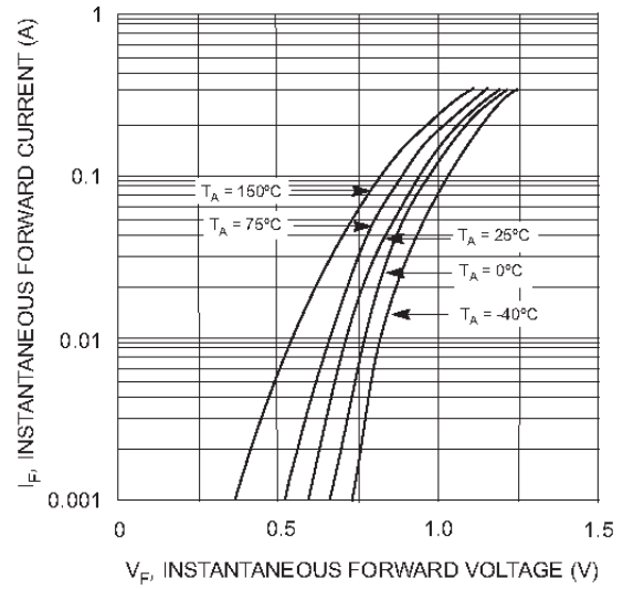
Fig. 2 Forward Characteristics
