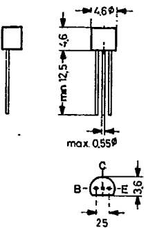
TO-92 Plastic Package Pin in-Line "D" Weight approx. 0.18 g
