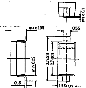
60A2 Diode Plastic Package Weight approx. 0.013 g
