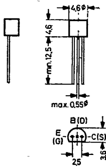
TO-92 Plastic Package (10D3) Pin in-Line "B" Weight approx. 0.18 g
