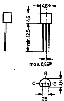
TO-92 Plastic Package Pin in-Line "E" Weight approx. 0.18 g
