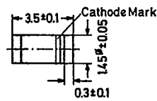
MiniMELF Glass Case Weight approx. 0.05 g
