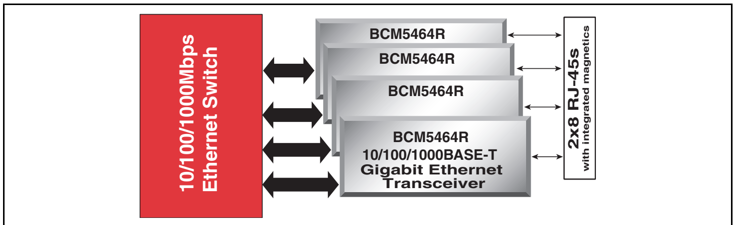
BCM5464R System Diagram
