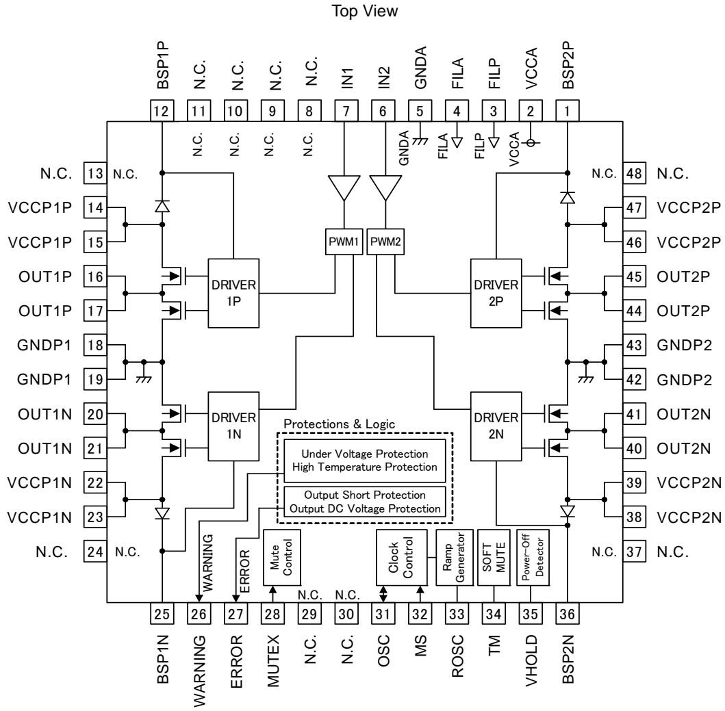
Fig. 22 Pin Assignment Diagram
