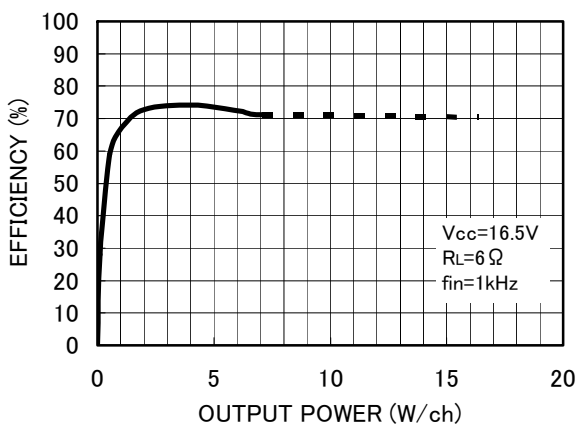
Fig. 20 Efficiency - Output power
