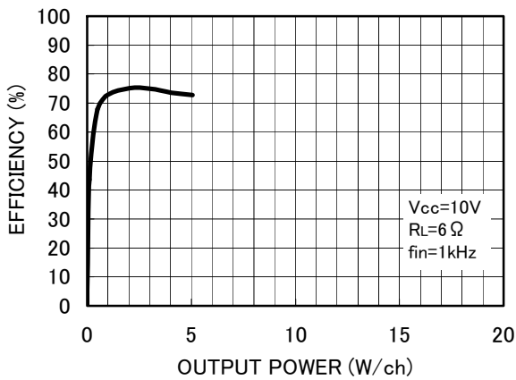
Fig. 18 Efficiency - Output power
