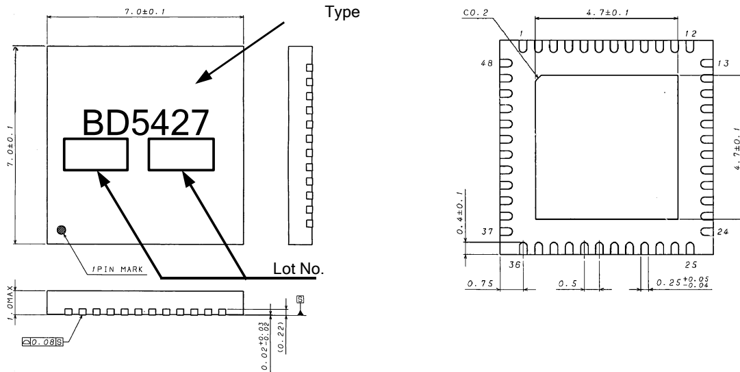
Fig. 23 Outer Dimensions and Inscriptions of VQFN048V7070 Package
