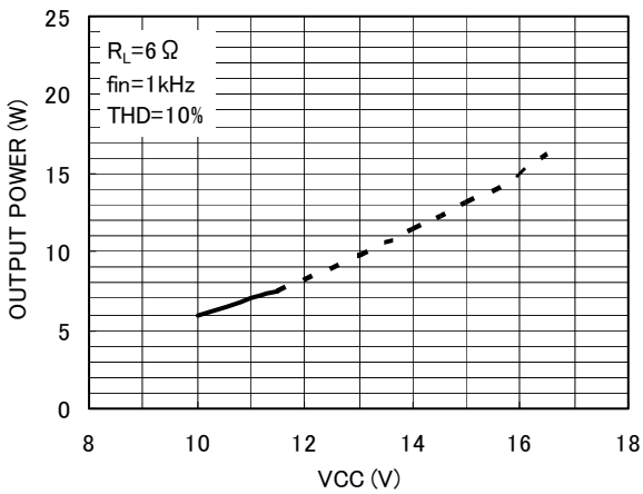
Fig. 17 Output power - Power supply voltage
