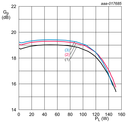
V_{DS} = 28\text{ V}; I_{DQ} = 700\text{ mA}; t_p = 100\text{ }\mu\text{s}; \delta = 10\text{ }\% . (1) f = 1807.5\text{ MHz} (2) f = 1840.0\text{ MHz} (3) f = 1872.5\text{ MHz}
