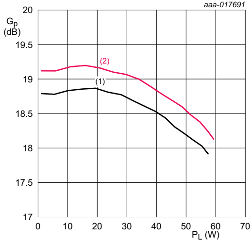
V_{DS} = 28\text{ V}; I_{Dq} = 700\text{ mA}; 5\text{ MHz carrier spacing.} (1) f = 1810\text{ MHz} (2) f = 1875\text{ MHz}
