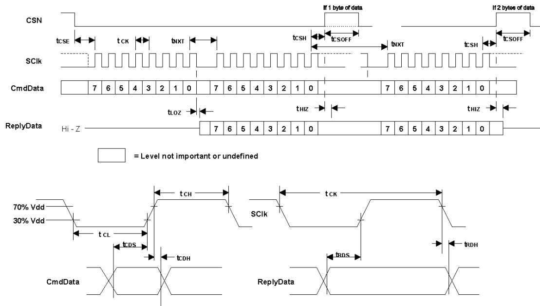
Figure 13 C-BUS Timing
