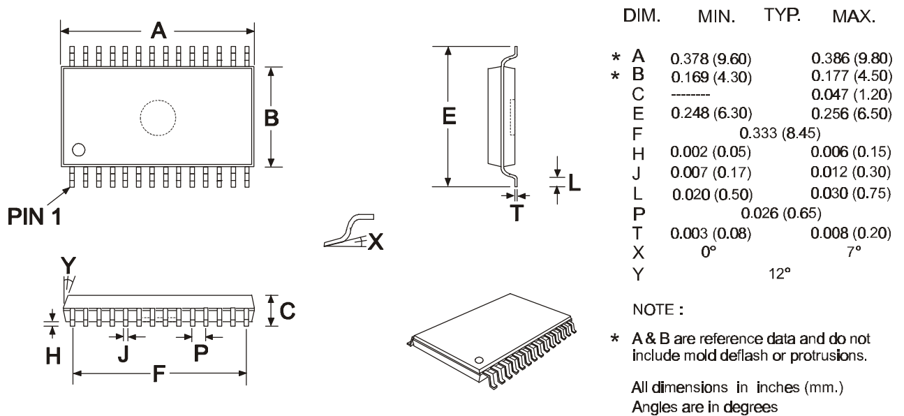
Figure 15 Mechanical Outline of 28-pin TSSOP (E1): Order as part no. CMX883E1
