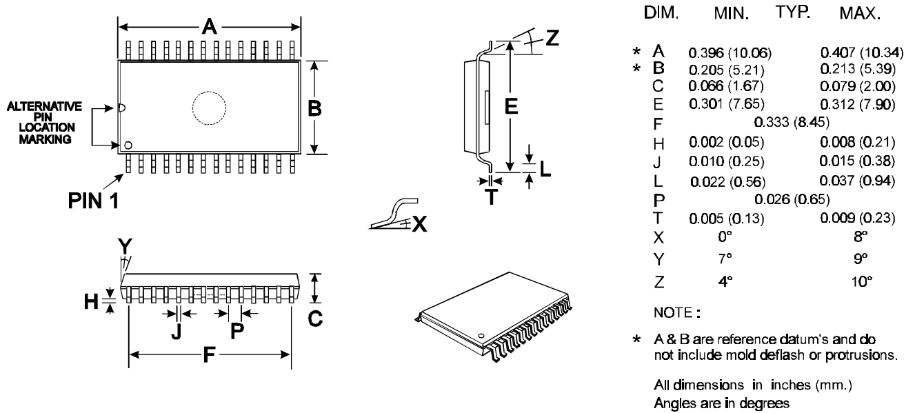
Figure 14 Mechanical Outline of 28-pin SSOP (D6): Order as part no. CMX883D6
