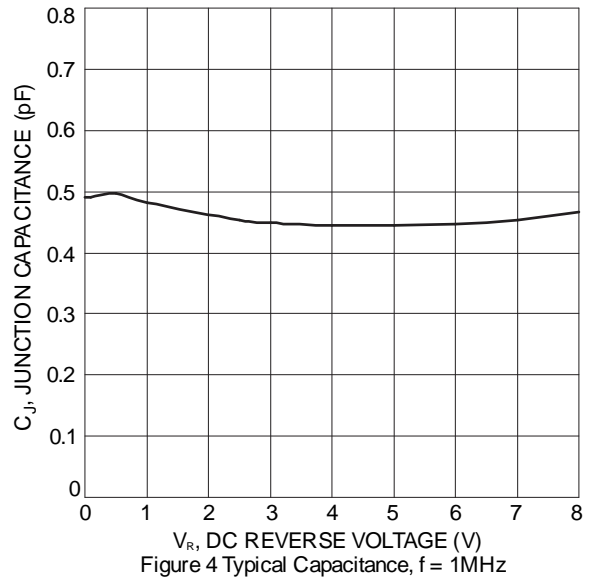
Figure 4 Typical Capacitance, f = 1MHz
