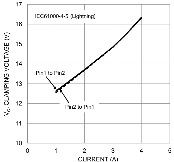
Figure 6 Clamping Voltage Characteristic (tp=8/20µs)
