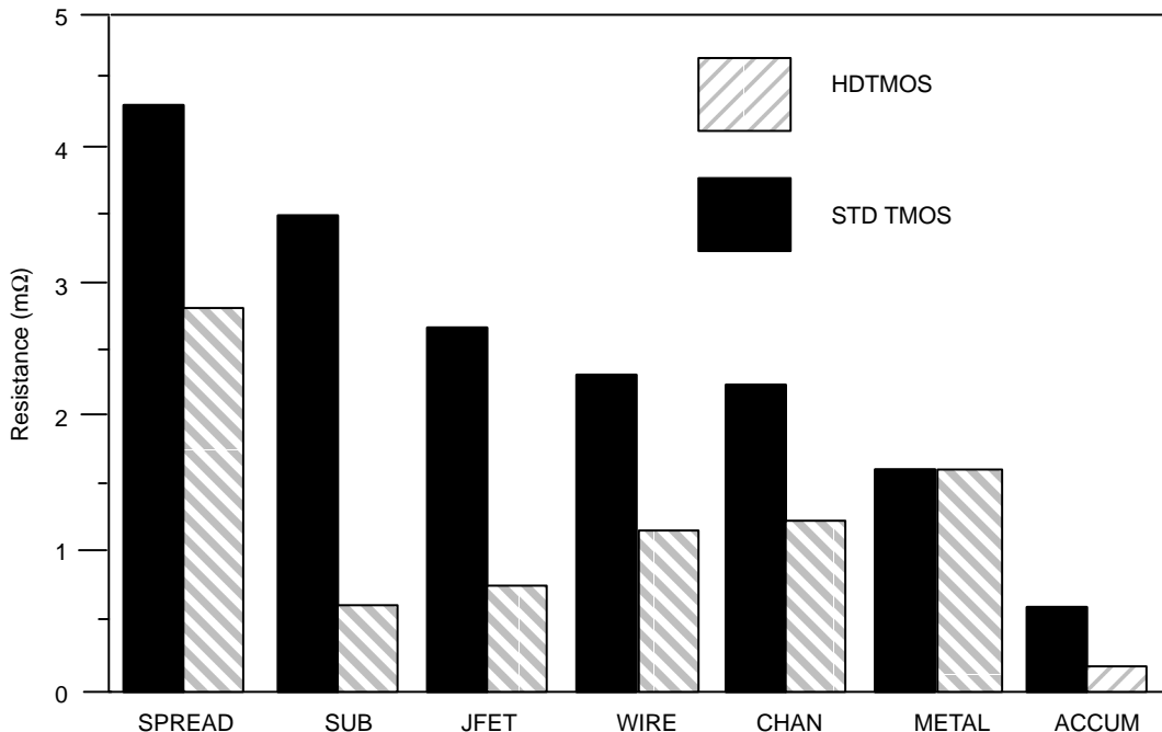
Figure 3. On-Resistance Components
