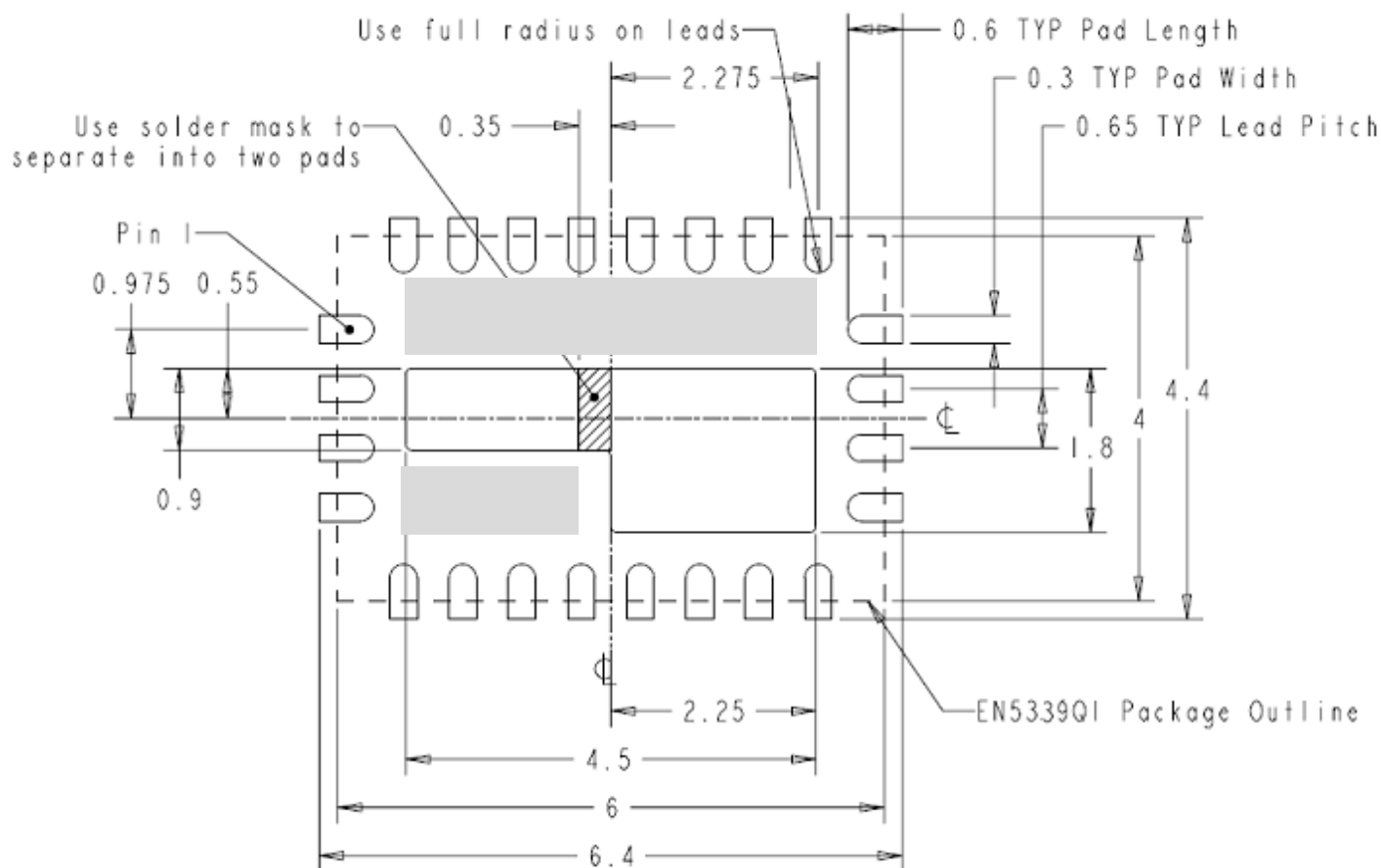
Figure 10. Recommended Footprint for PCB (Top View)
