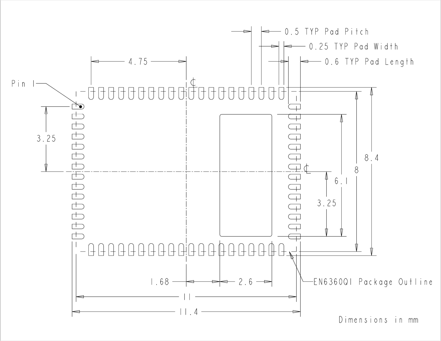
Figure 12: EN6360QI PCB Footprint (Top View)
