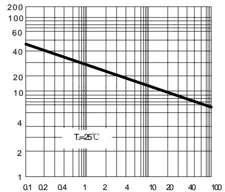
FIG.4-TYPICAL JUNCTION CAPACITANCE
