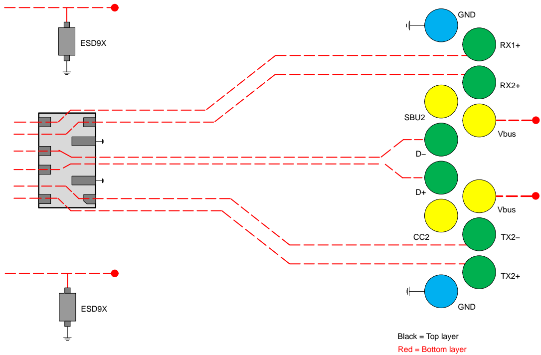
Figure 17. USB 3.1 Type-C Layout Diagram
