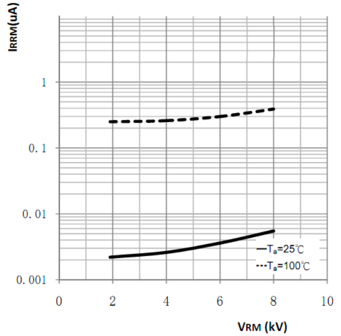
Fig2 Reverse Characteristics
