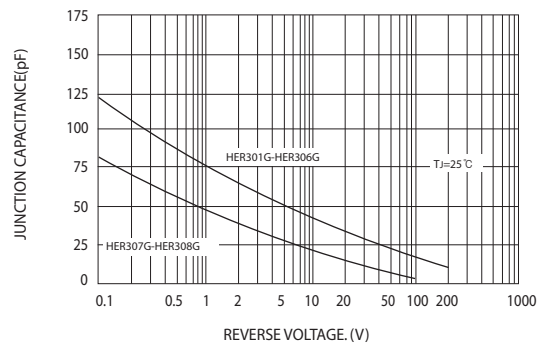
FIG.6-TYPICAL JUNCTION CAPACITANCE
