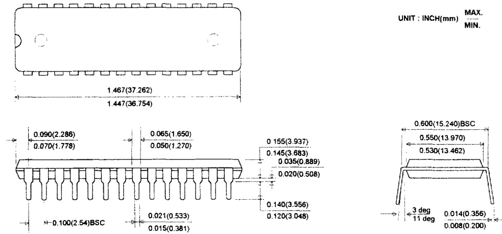
28pin 600mil Dual In-Line Package(P)
