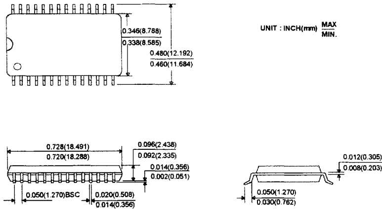
28pin 330mil Small Outline Package(J)
