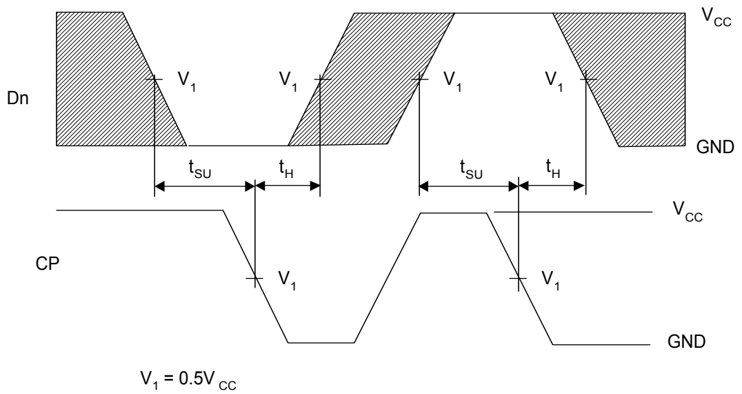
Figure 2 - Time diagram
