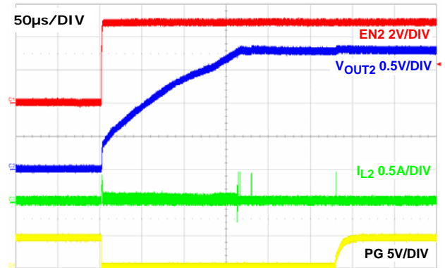
FIGURE 26. SOFT-START AT NO LOAD CHANNEL 2 (PFM)
