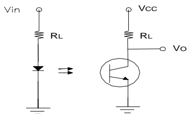
Test Circuit
