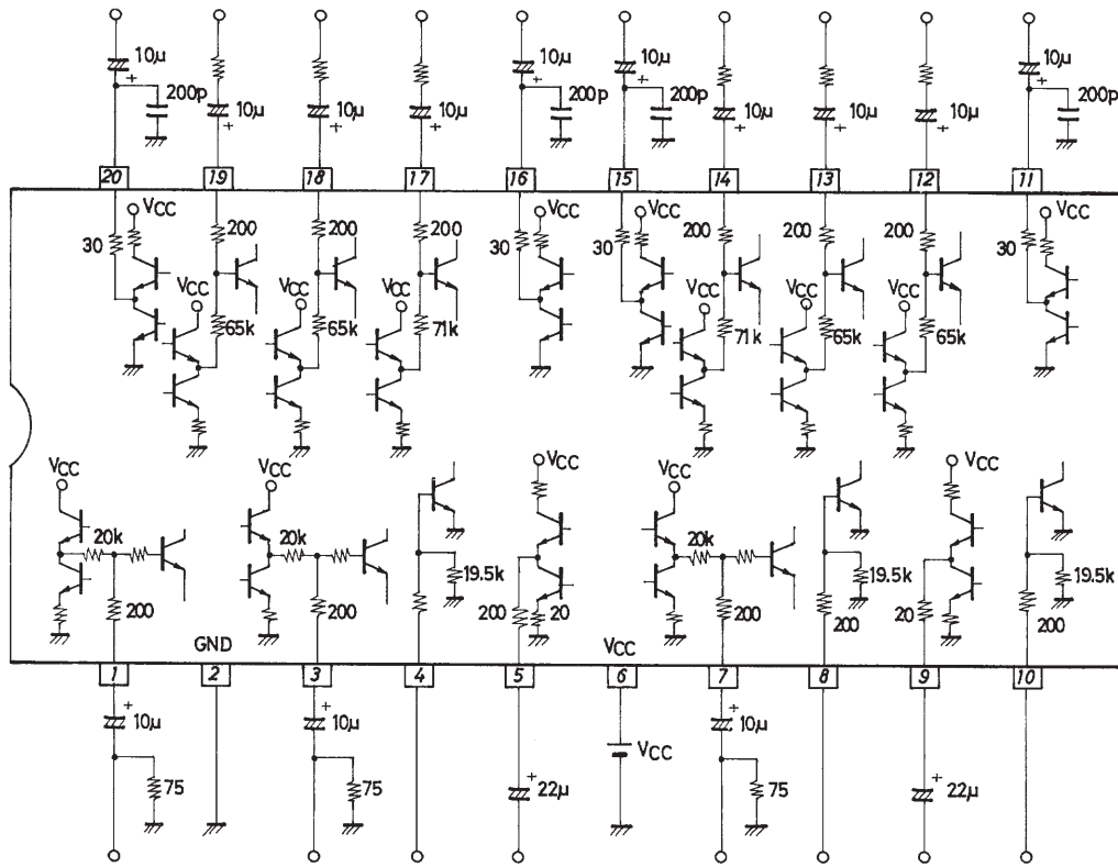
Unit ( resistance:Ω, capacitance:F )
