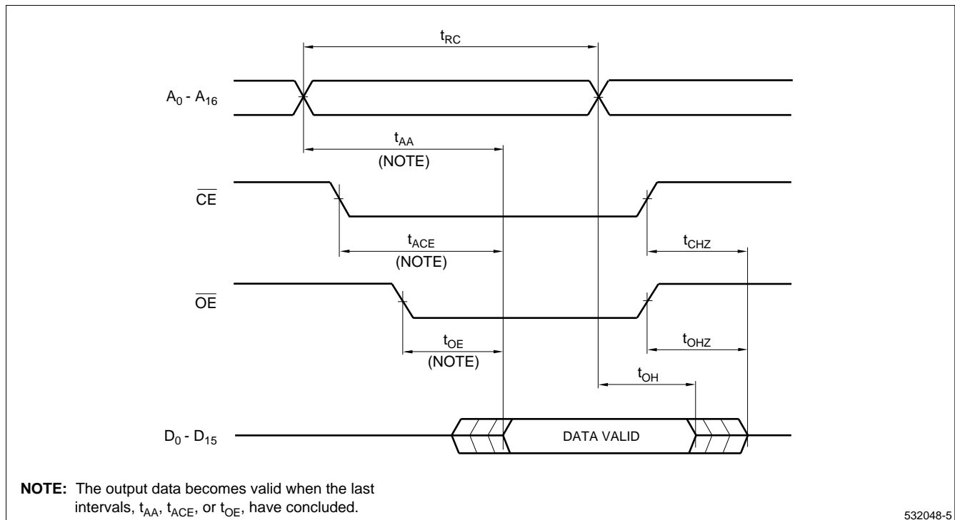
Figure 5. Timing Diagram
