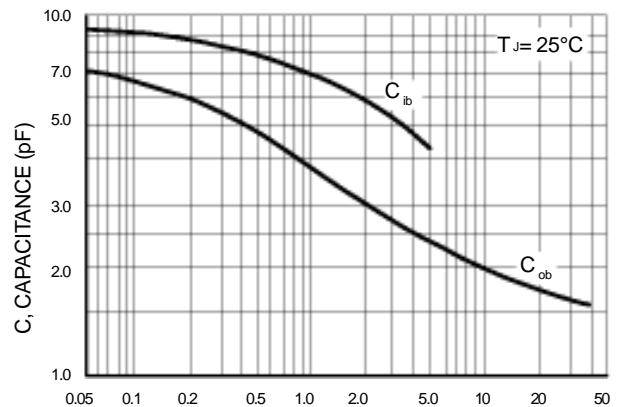
Figure 13. Capacitance
