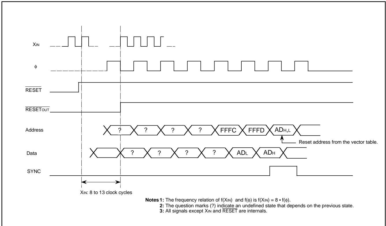
Fig. 50 Reset sequence
