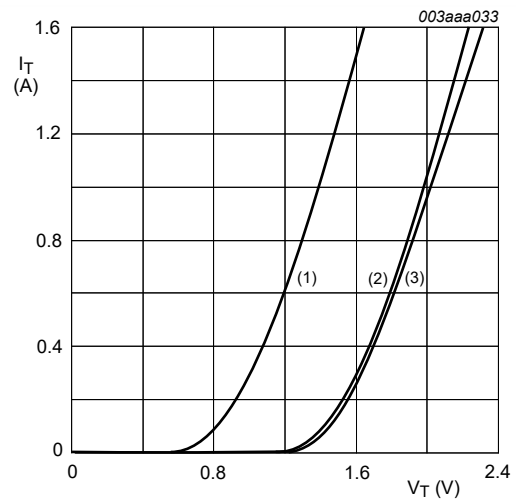
V_o = 1.45\text{ V}; R_s = 0.1875\ \Omega Fig. 10. On-state current as a function of on-state voltage
