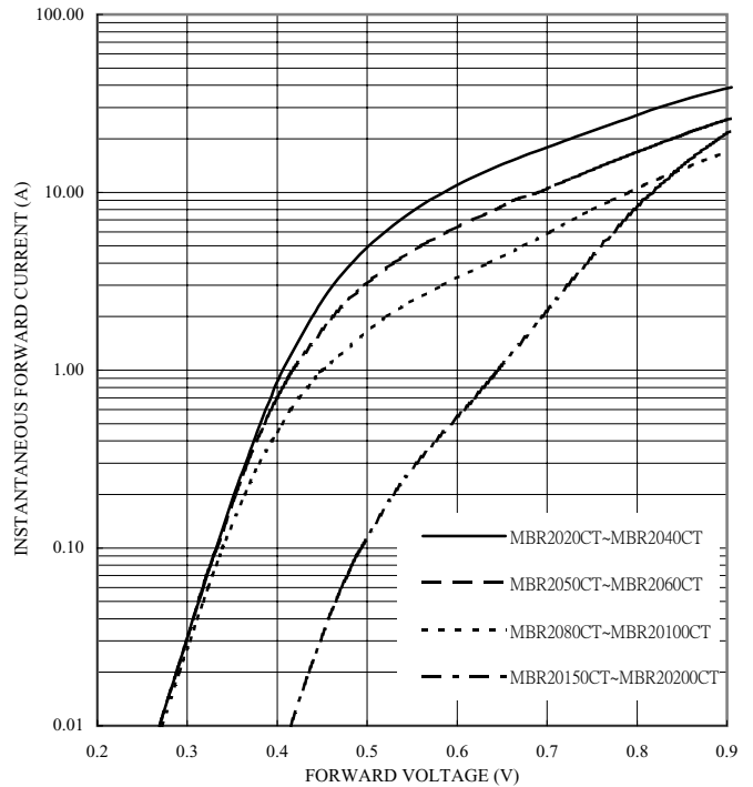
FIG. 2-TYPICAL FORWARD CHARACTERISTICS
