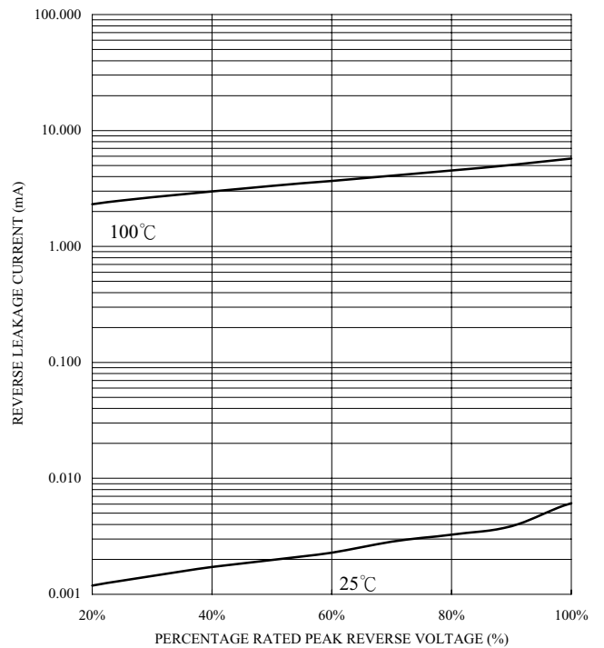
FIG. 5-TYPICAL REVERSE CHARACTERISTICS
