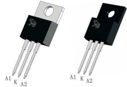
TO-220
