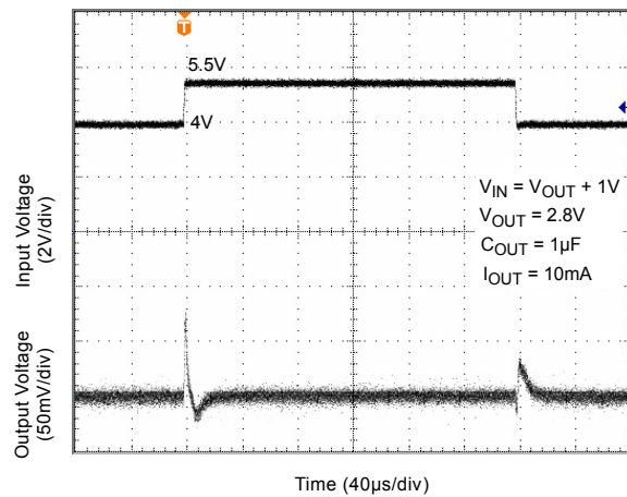
Line Transient
