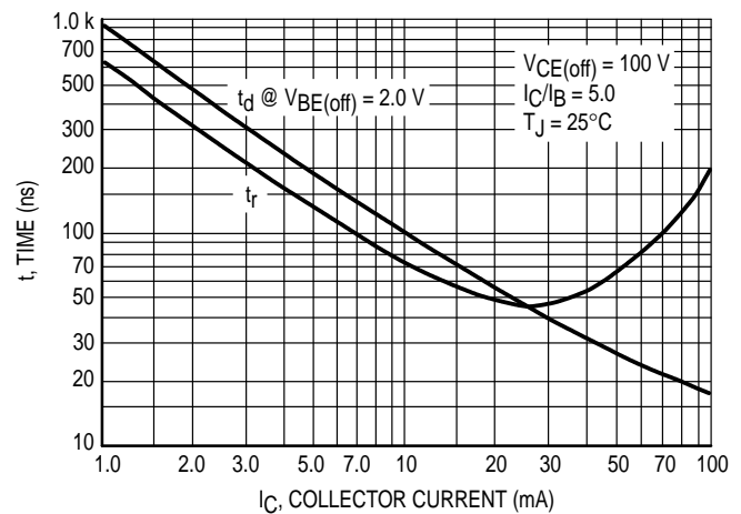
Figure 6. Turn-On Time
