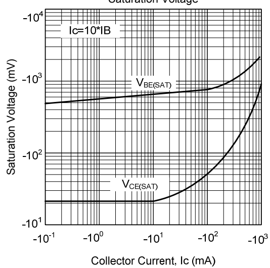
Saturation Voltage
