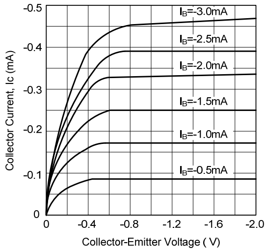
Static Characteristics
