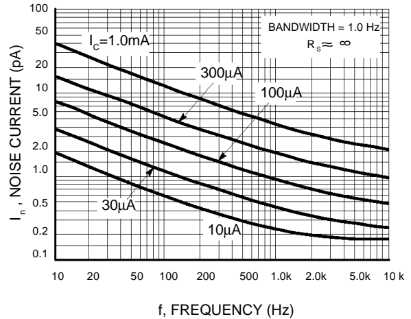
Figure 4. Noise Current
